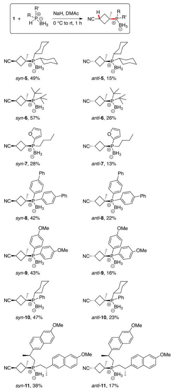
Scheme 3. Hydrophosphination of Nitrile 1 with Various Phosphine Boranes
