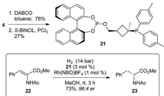
Scheme 7. Preparation of Bidentate Phosphine Ligand 21 and Asymmetric Hydrogenation of Dehydrophenylalanine 22
