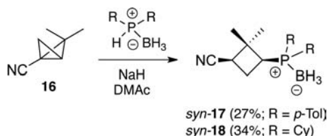
Scheme 6. Addition of H -Phosphonates to Bicyclo[1.1.0]butanes 1 and 16
