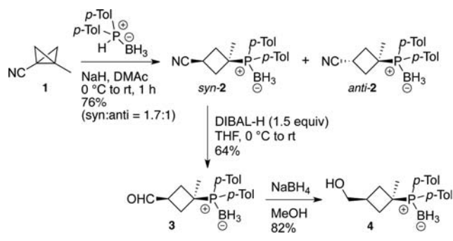
Scheme 2. Hydrophosphination of 3-Methylbicyclo[1.1.0]butane-1-carbonitrile 1 and Transformation to Phosphine Borane Alcohol 4
